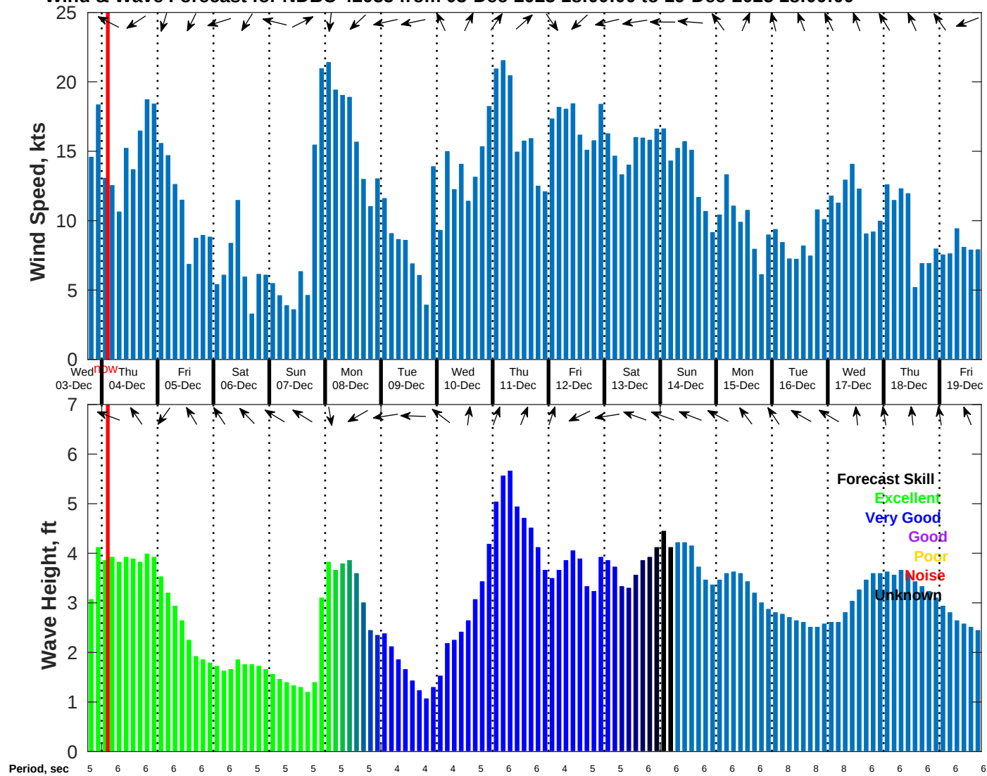
Wind & Wave Forecast for NDBC 42035 from 03-Dec-2025 18:00:00 to 19-Dec-2025 18:00:00
