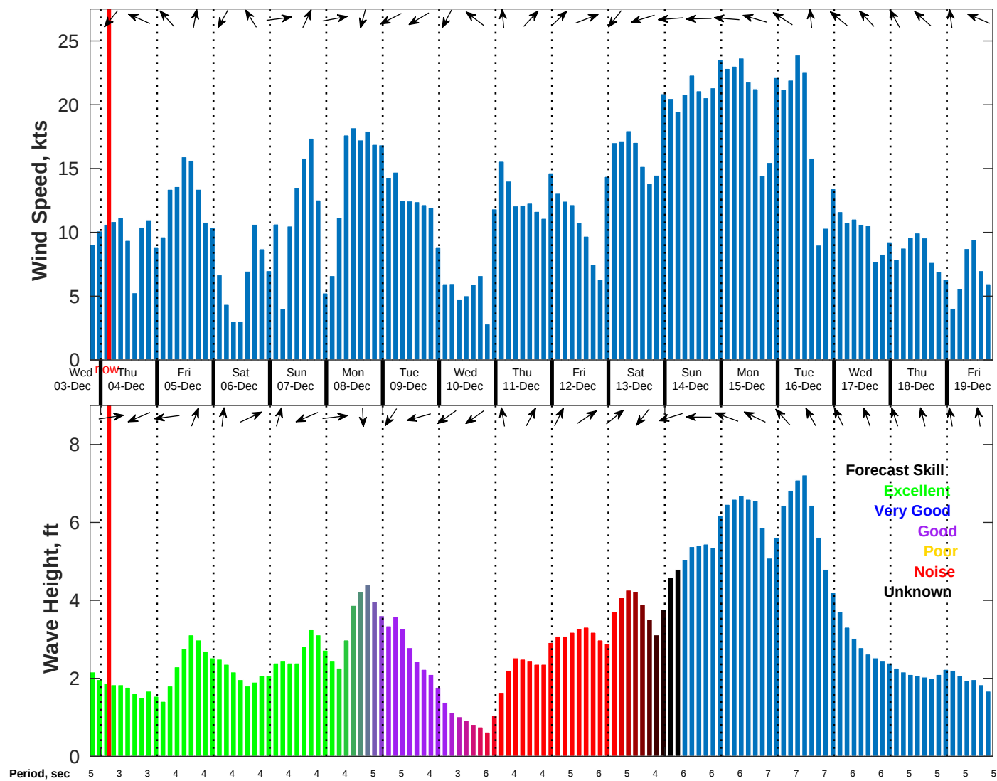
Wind & Wave Forecast for NDBC 42036 from 03-Dec-2025 19:00:00 to 19-Dec-2025 19:00:00
