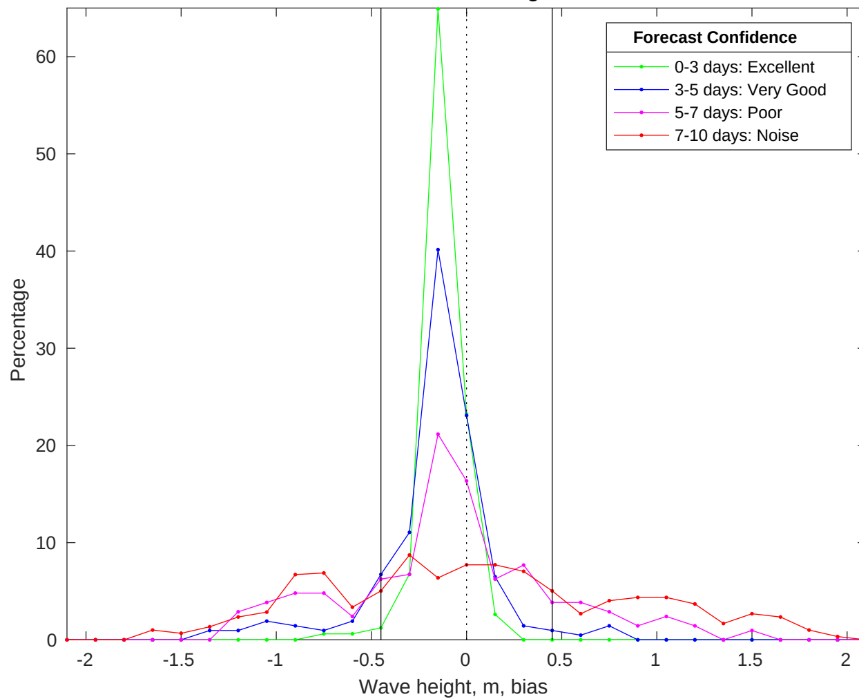
NDBC 42040 vs CMEMS Waves Bias Histogram: 04-Dec-2025
