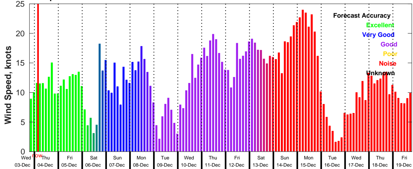
GFS Wind Speed Forecast for NDBC 42040 from 03-Dec-2025 19:00:00 to 19-Dec-2025 19:00:00
