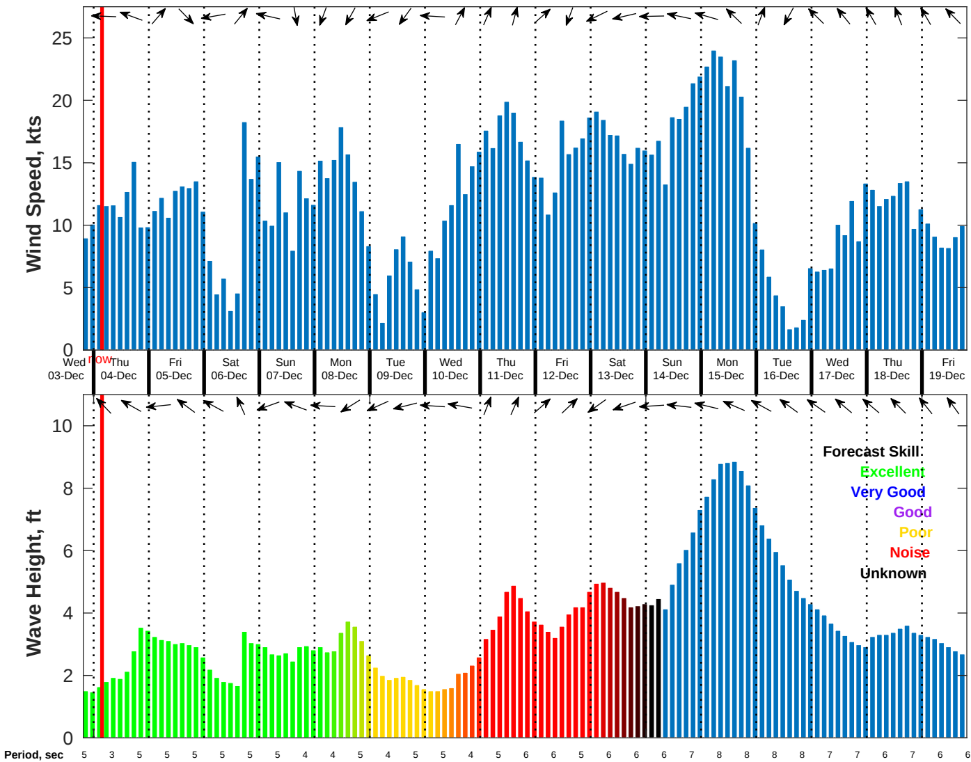
Wind & Wave Forecast for NDBC 42040 from 03-Dec-2025 19:00:00 to 19-Dec-2025 19:00:00
