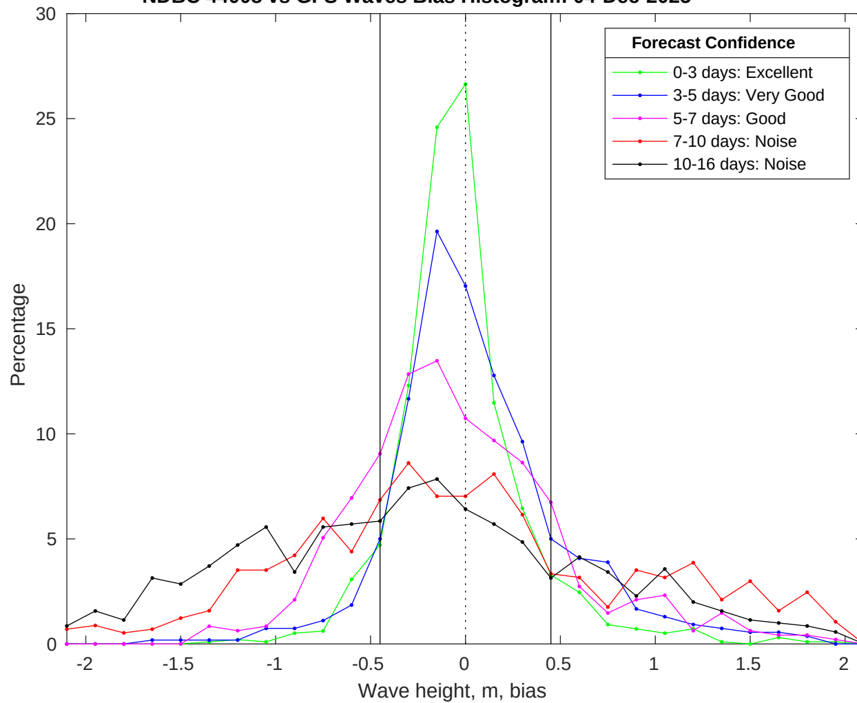
NDBC 44008 vs GFS Waves Bias Histogram: 04-Dec-2025
