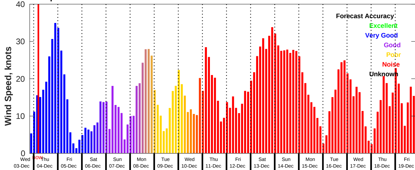
GFS Wind Speed Forecast for NDBC 44008 from 03-Dec-2025 20:00:00 to 19-Dec-2025 20:00:00
