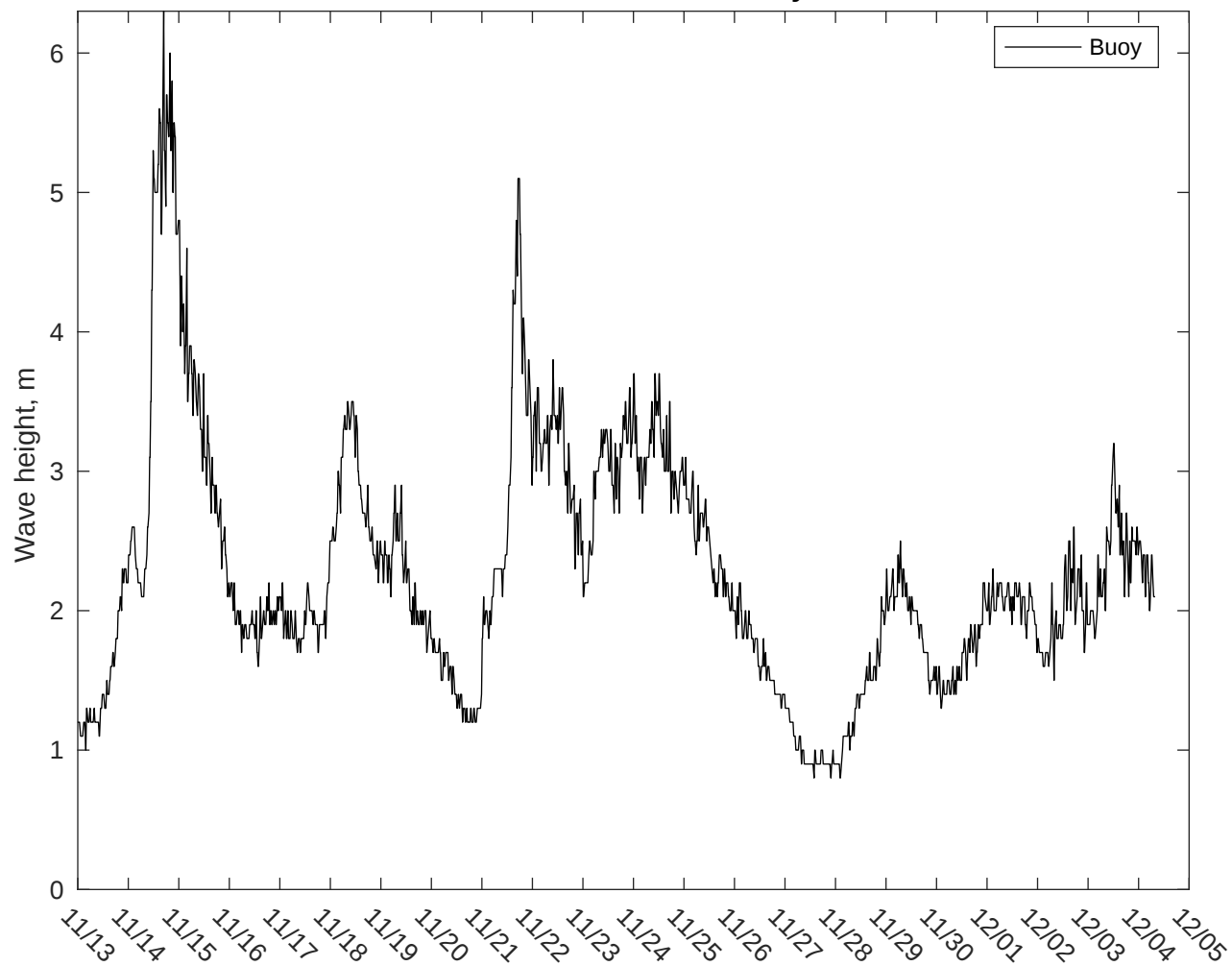
NDBC 46011 vs CMEMS Waves: 10 to 16 day forecast
