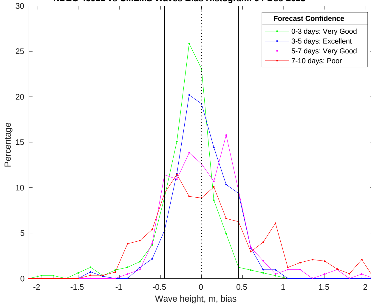
NDBC 46011 vs CMEMS Waves Bias Histogram: 04-Dec-2025
