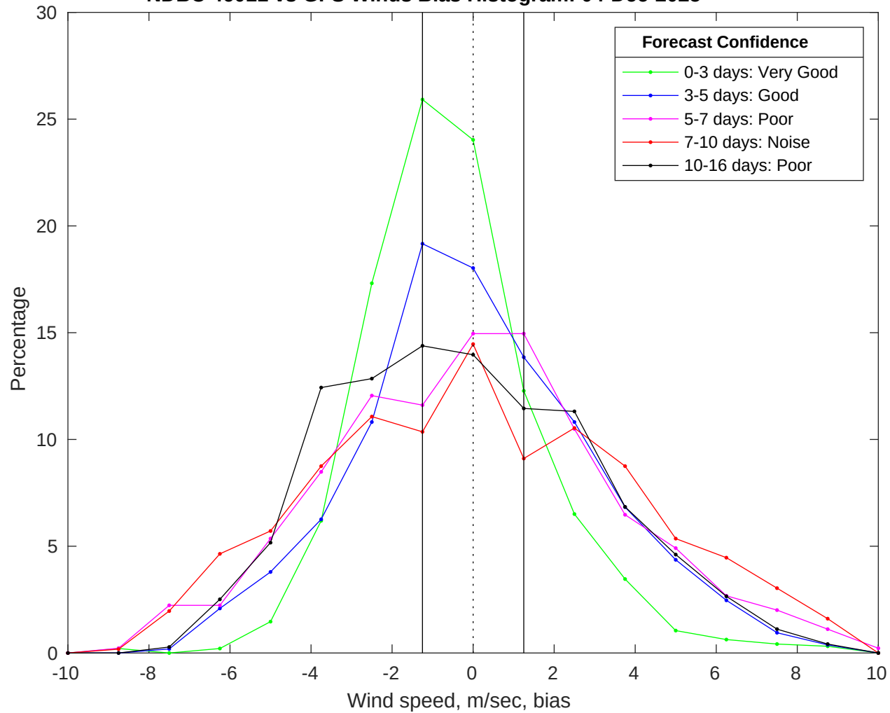
NDBC 46011 vs GFS Winds Bias Histogram: 04-Dec-2025
