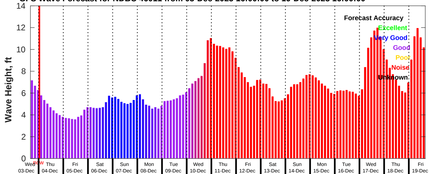
GFS Wave Forecast for NDBC 46011 from 03-Dec-2025 16:00:00 to 19-Dec-2025 16:00:00
