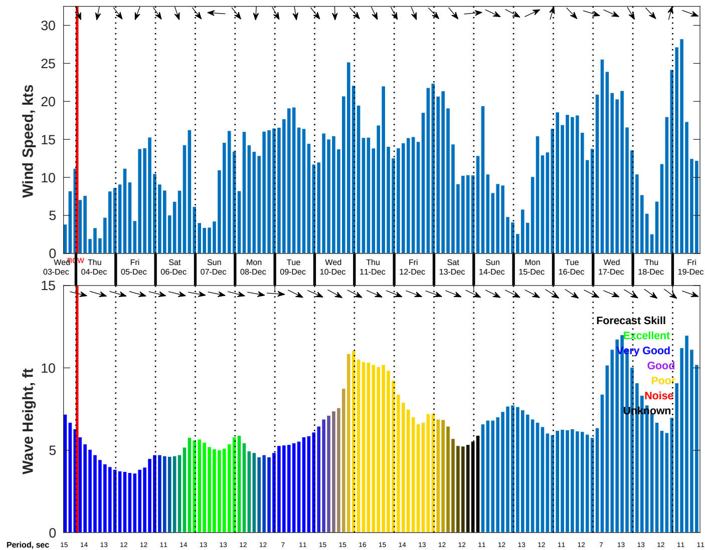
Wind & Wave Forecast for NDBC 46011 from 03-Dec-2025 16:00:00 to 19-Dec-2025 16:00:00
