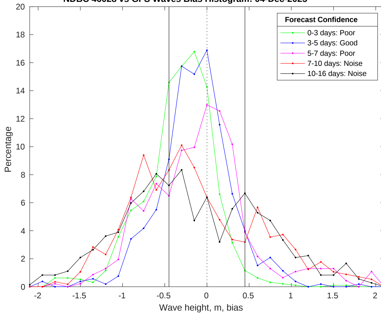
NDBC 46028 vs GFS Waves Bias Histogram: 04-Dec-2025
