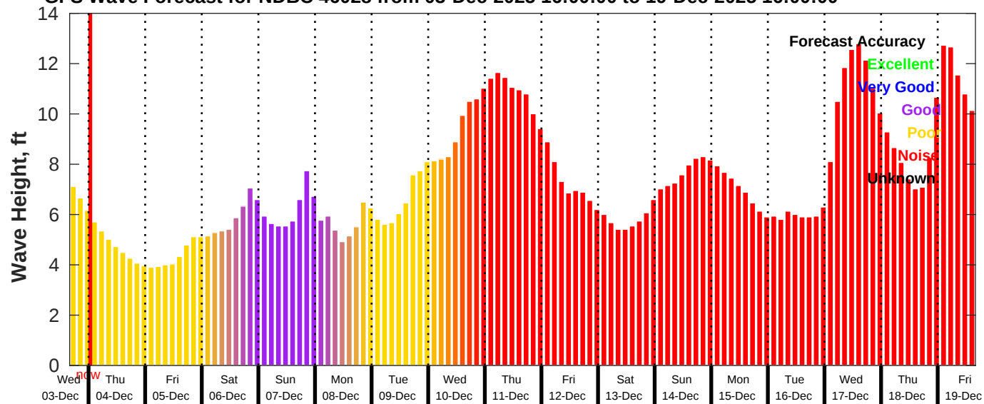
GFS Wave Forecast for NDBC 46028 from 03-Dec-2025 16:00:00 to 19-Dec-2025 16:00:00
