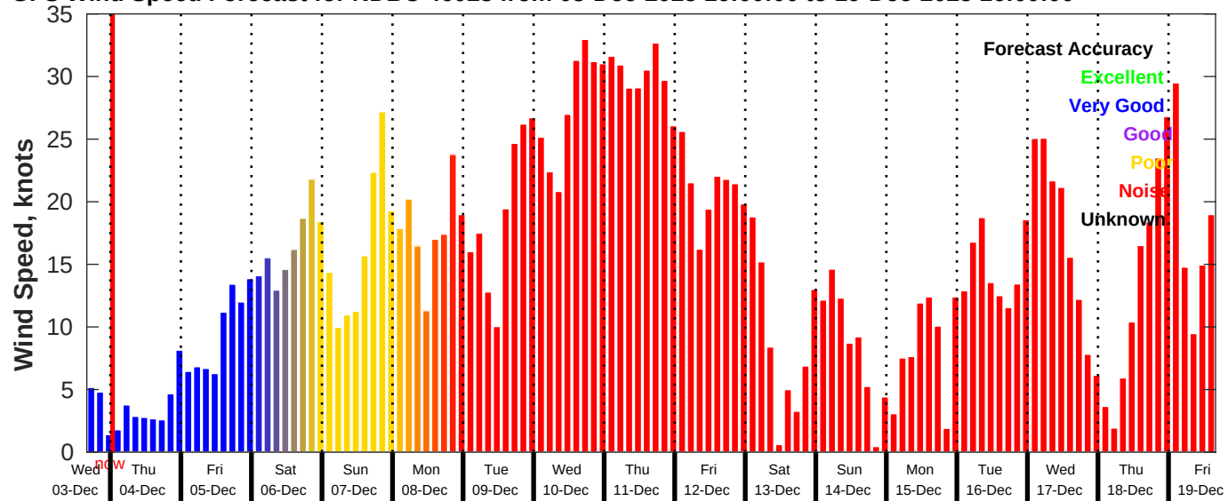
GFS Wind Speed Forecast for NDBC 46028 from 03-Dec-2025 16:00:00 to 19-Dec-2025 16:00:00
