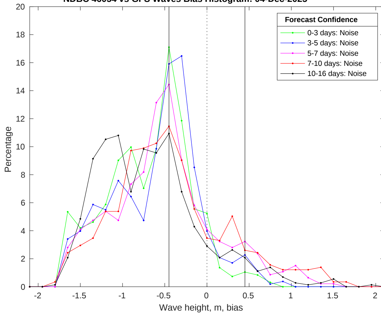
NDBC 46054 vs GFS Waves Bias Histogram: 04-Dec-2025
