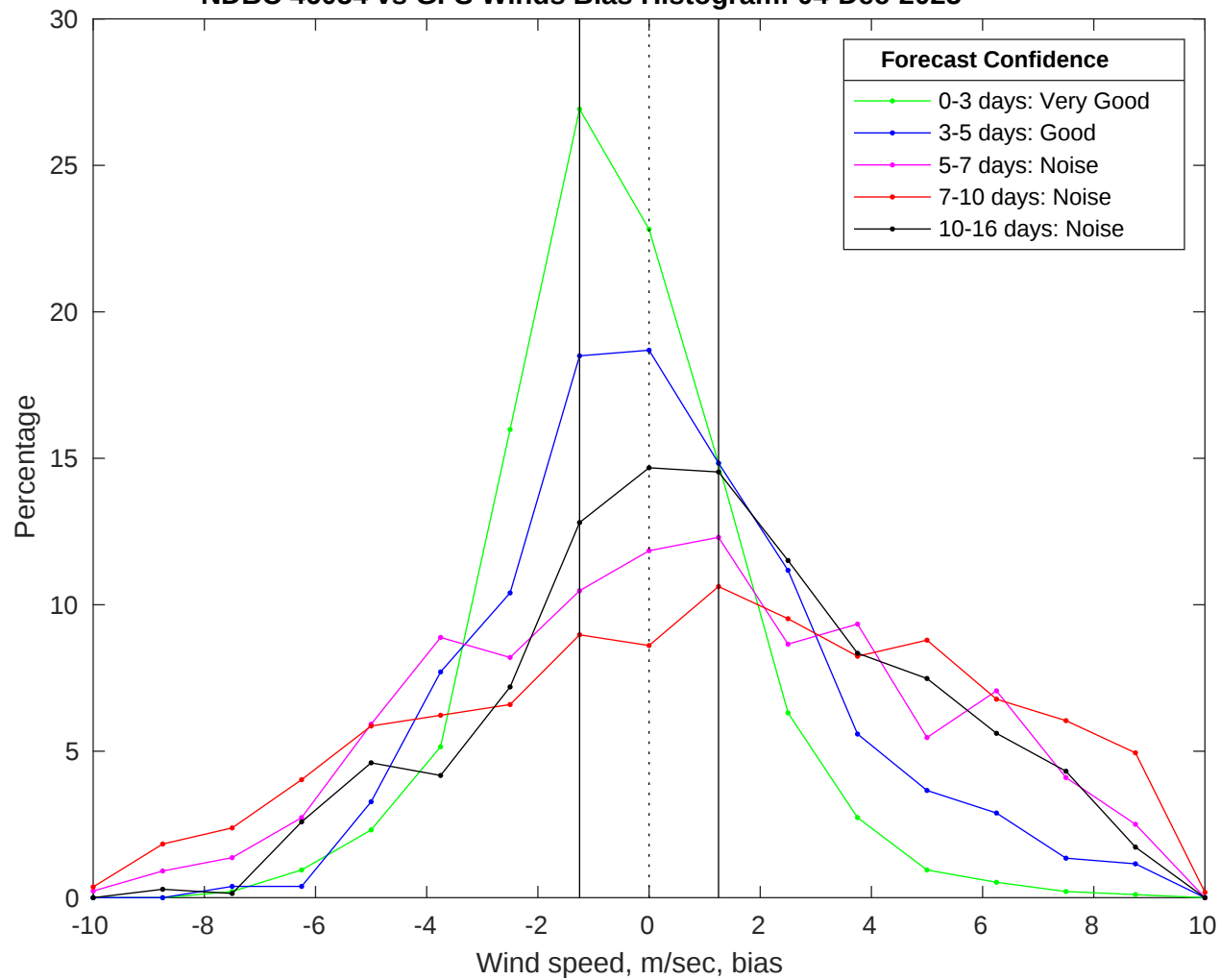
NDBC 46054 vs GFS Winds Bias Histogram: 04-Dec-2025
