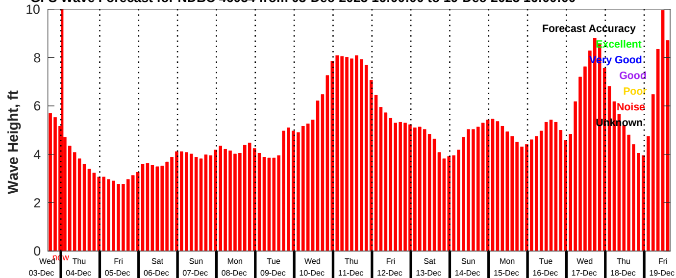
GFS Wave Forecast for NDBC 46054 from 03-Dec-2025 16:00:00 to 19-Dec-2025 16:00:00
