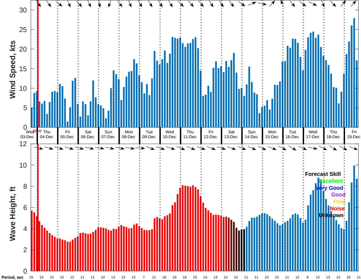
Wind & Wave Forecast for NDBC 46054 from 03-Dec-2025 16:00:00 to 19-Dec-2025 16:00:00
