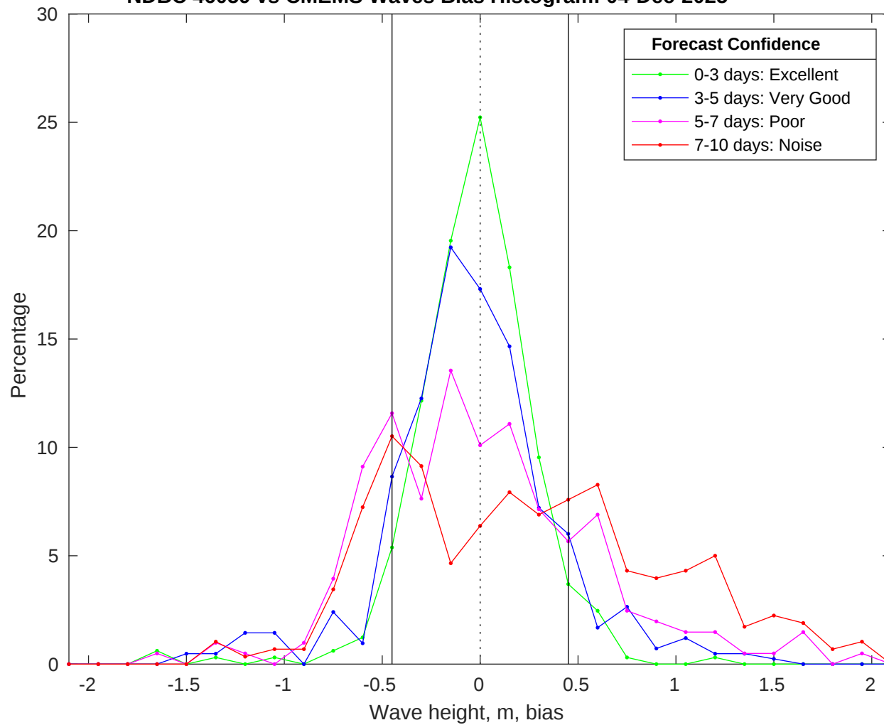
NDBC 46059 vs CMEMS Waves Bias Histogram: 04-Dec-2025
