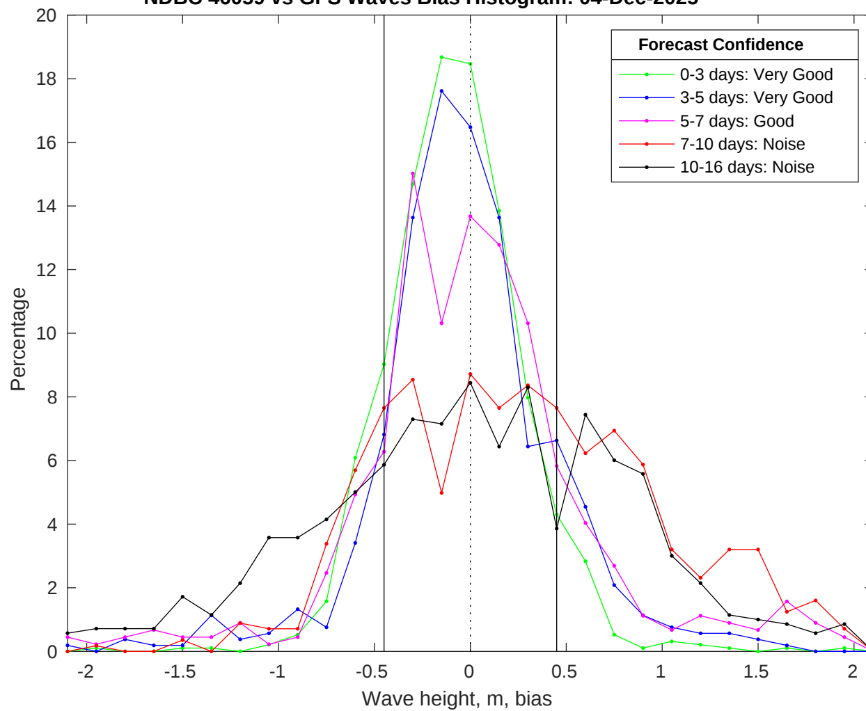
NDBC 46059 vs GFS Waves Bias Histogram: 04-Dec-2025
