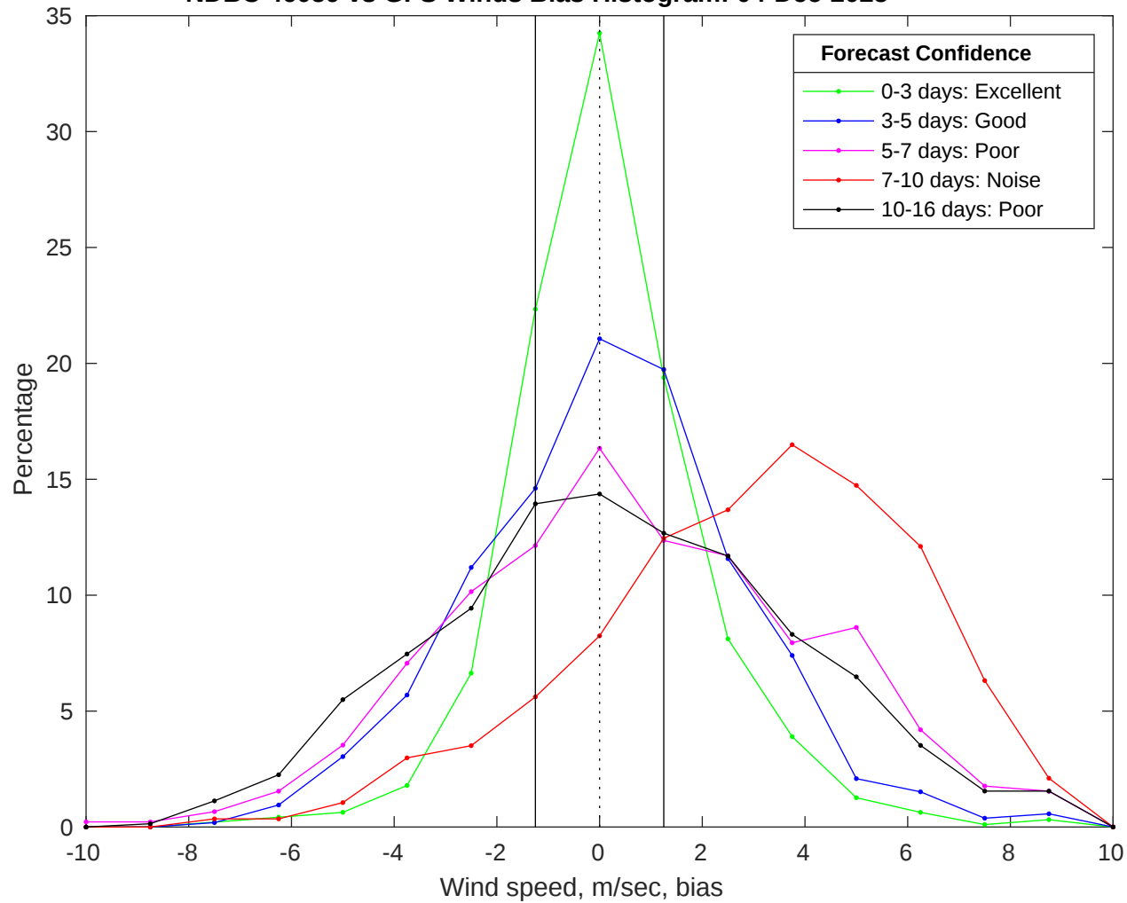
NDBC 46059 vs GFS Winds Bias Histogram: 04-Dec-2025
