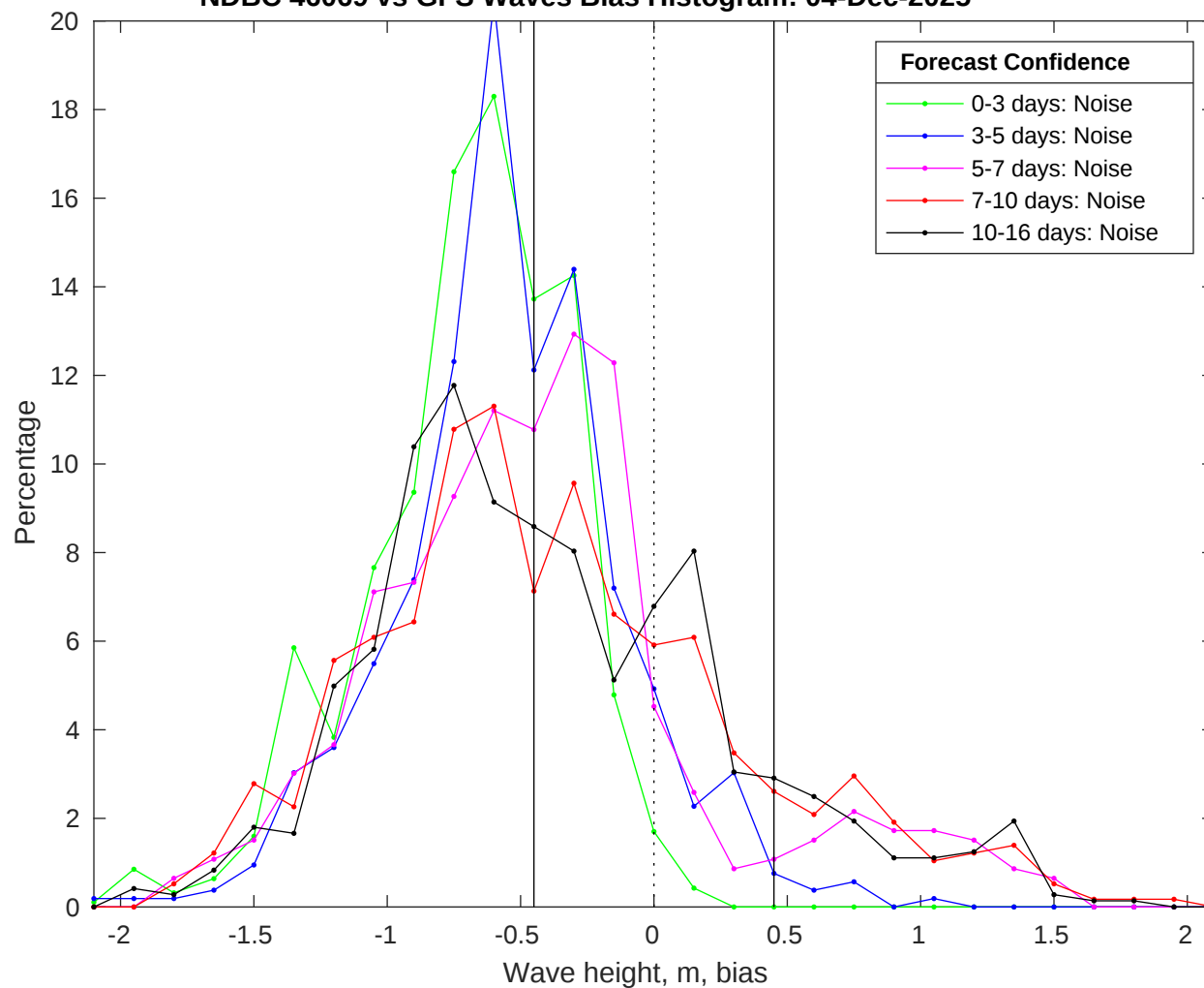
NDBC 46069 vs GFS Waves Bias Histogram: 04-Dec-2025
