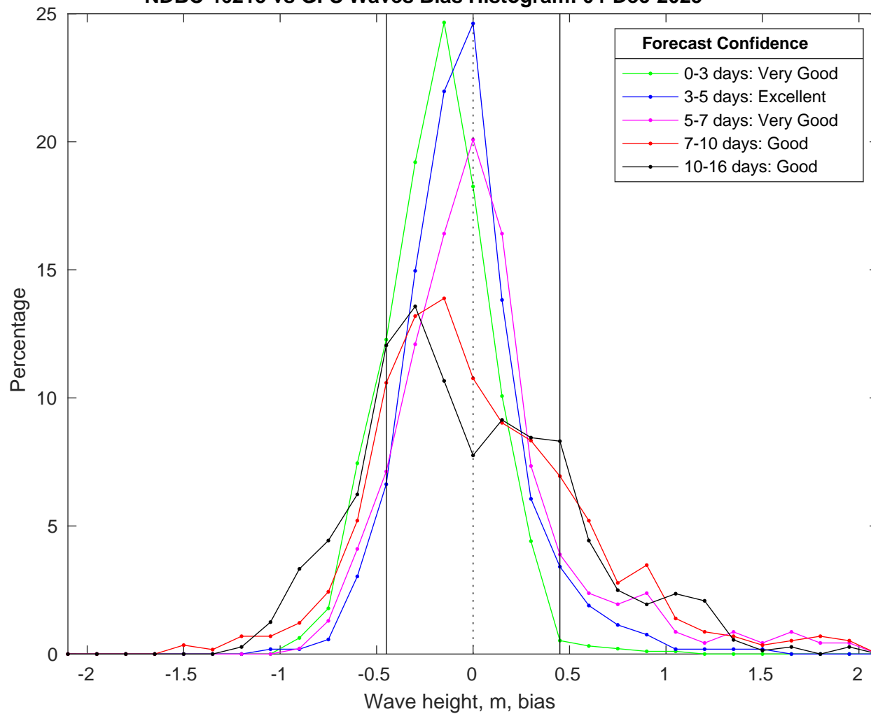
NDBC 46215 vs GFS Waves Bias Histogram: 04-Dec-2025
