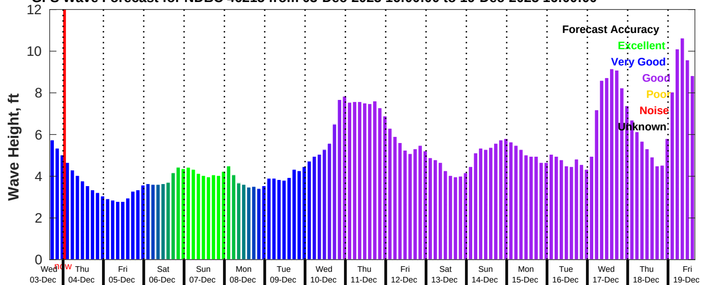
GFS Wave Forecast for NDBC 46215 from 03-Dec-2025 16:00:00 to 19-Dec-2025 16:00:00
