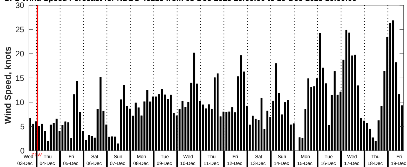
GFS Wind Speed Forecast for NDBC 46215 from 03-Dec-2025 16:00:00 to 19-Dec-2025 16:00:00
