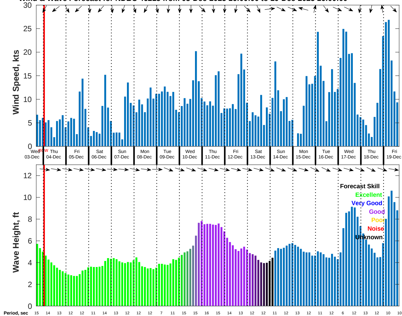
Wind & Wave Forecast for NDBC 46215 from 03-Dec-2025 16:00:00 to 19-Dec-2025 16:00:00
