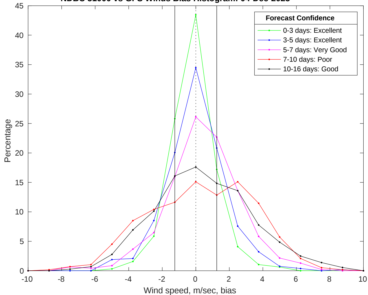
NDBC 51000 vs GFS Winds Bias Histogram: 04-Dec-2025
