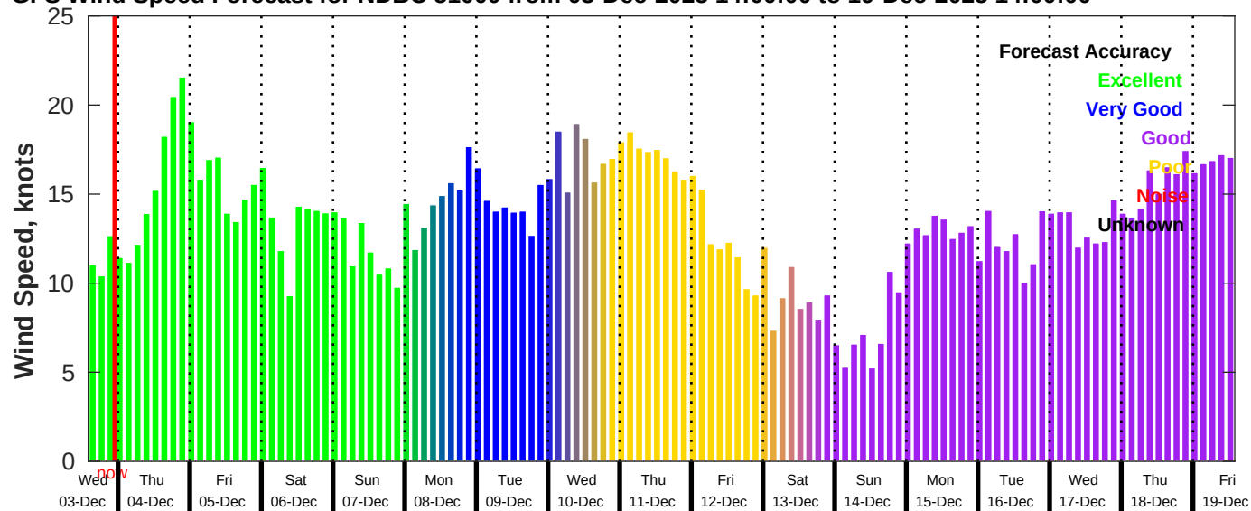
GFS Wind Speed Forecast for NDBC 51000 from 03-Dec-2025 14:00:00 to 19-Dec-2025 14:00:00
