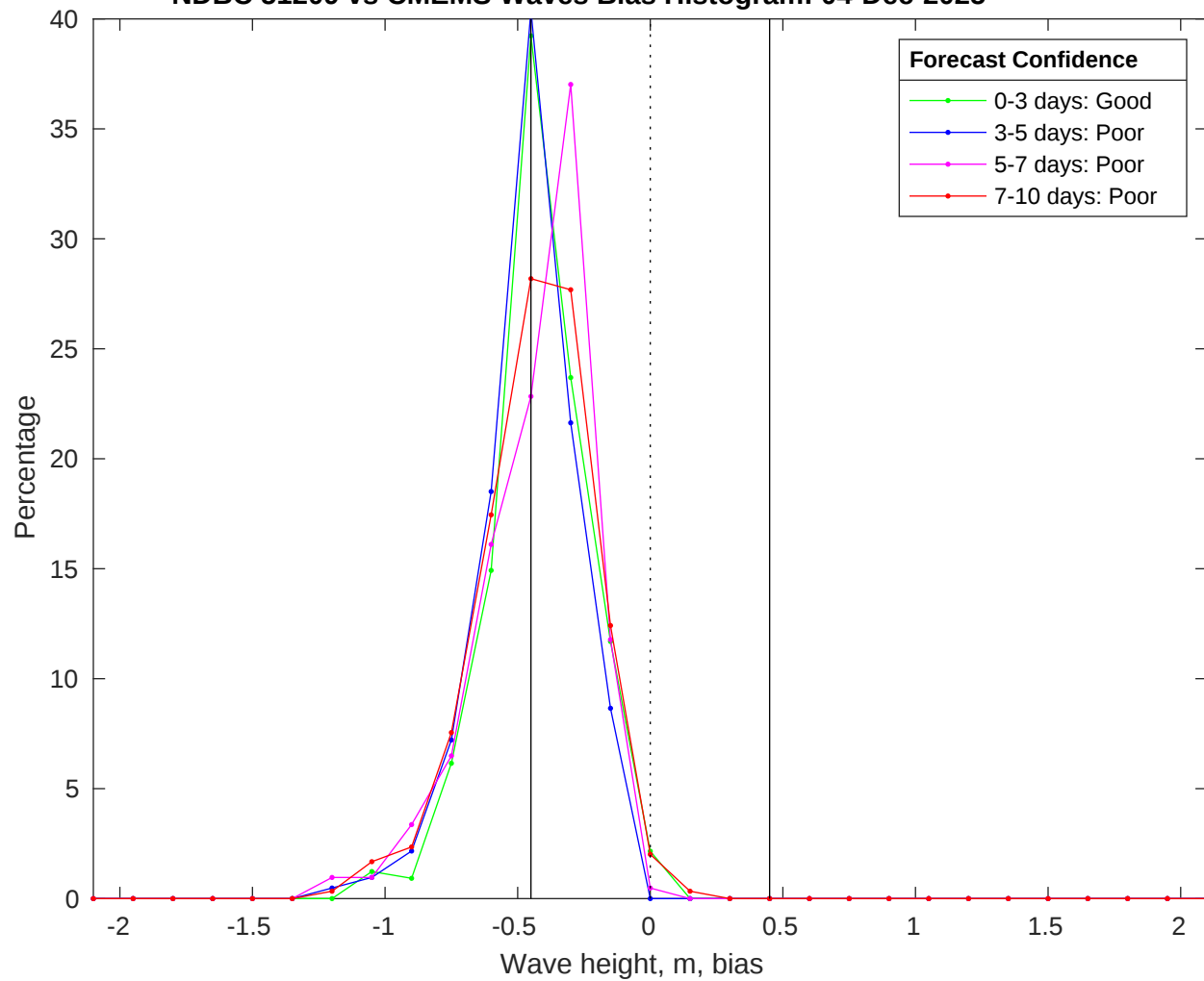
NDBC 51209 vs CMEMS Waves Bias Histogram: 04-Dec-2025
