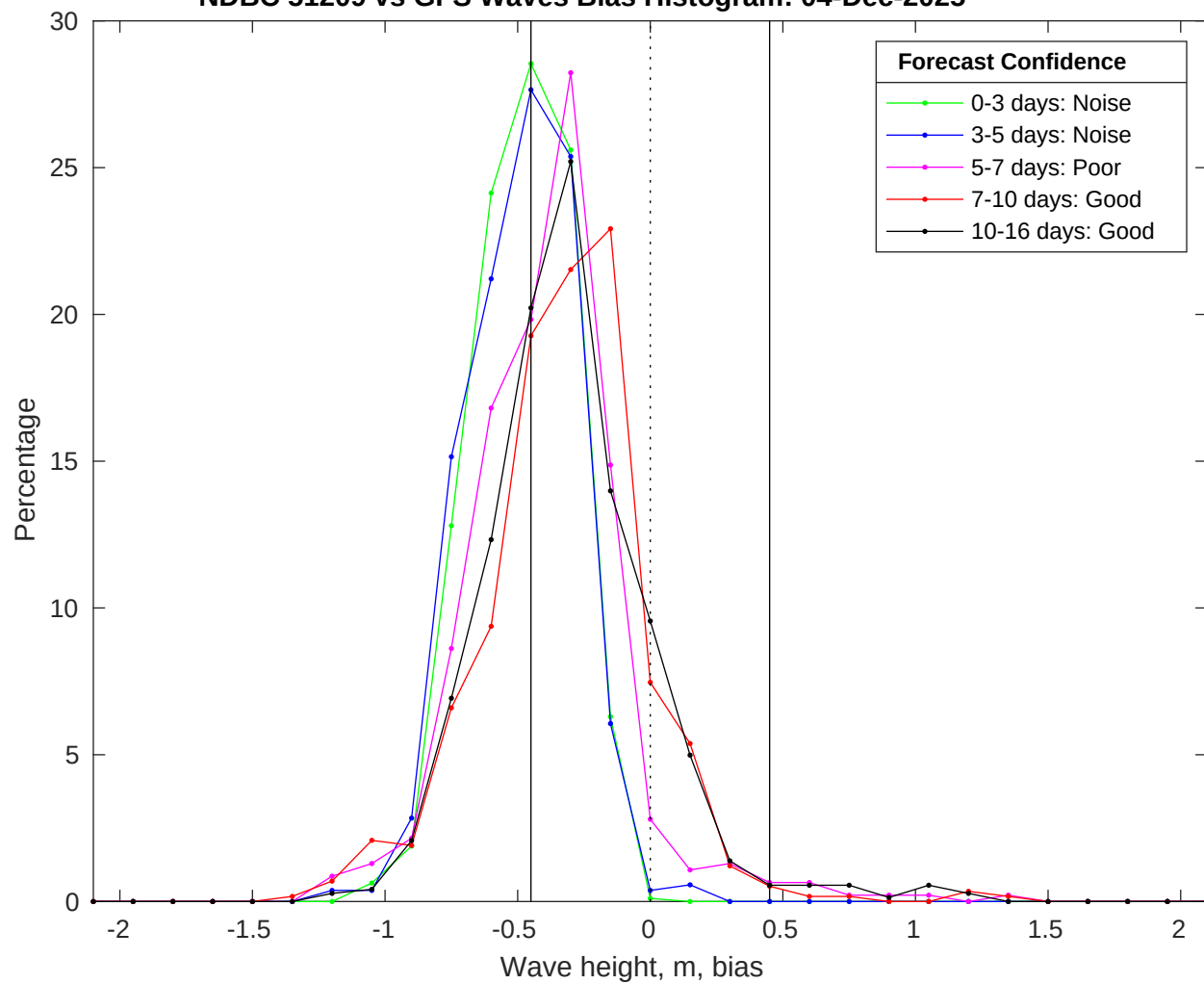
NDBC 51209 vs GFS Waves Bias Histogram: 04-Dec-2025
