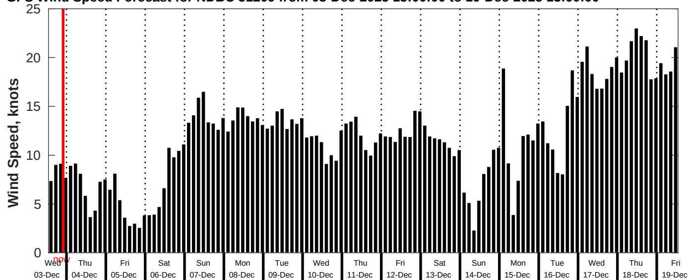
GFS Wind Speed Forecast for NDBC 51209 from 03-Dec-2025 13:00:00 to 19-Dec-2025 13:00:00
