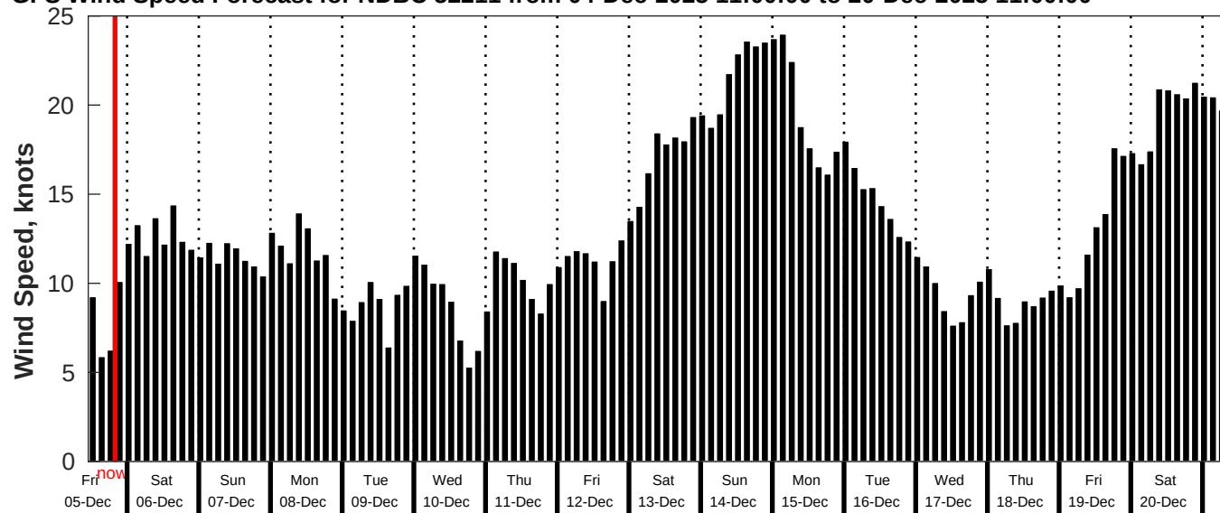
GFS Wind Speed Forecast for NDBC 52211 from 04-Dec-2025 11:00:00 to 20-Dec-2025 11:00:00
