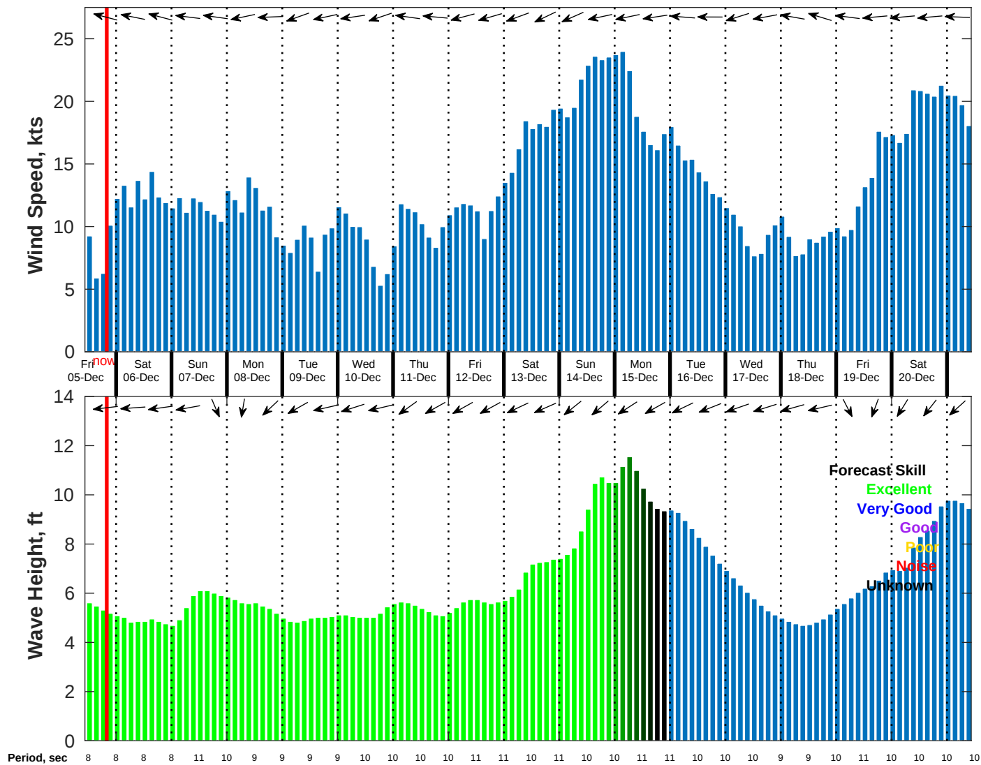
Wind & Wave Forecast for NDBC 52211 from 04-Dec-2025 11:00:00 to 20-Dec-2025 11:00:00
