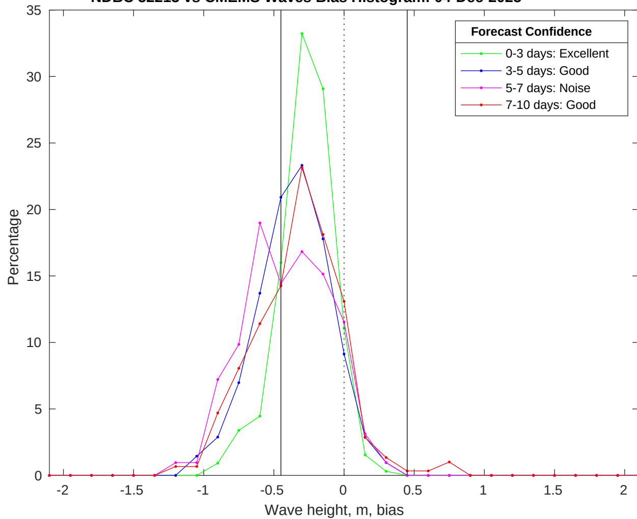
NDBC 52213 vs CMEMS Waves Bias Histogram: 04-Dec-2025
