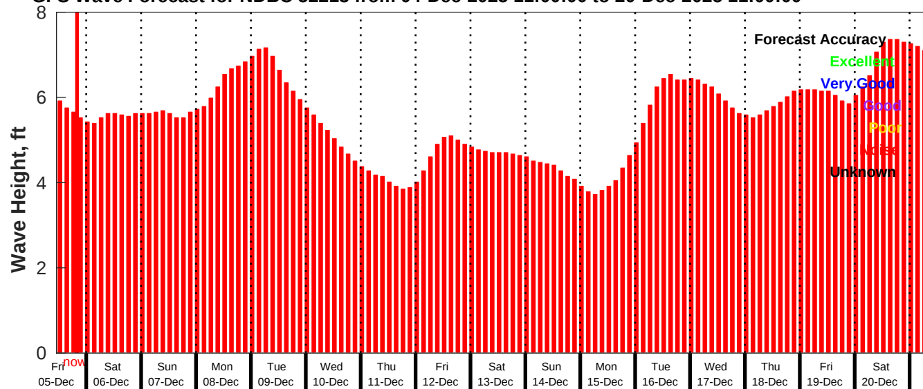
GFS Wave Forecast for NDBC 52213 from 04-Dec-2025 11:00:00 to 20-Dec-2025 11:00:00
