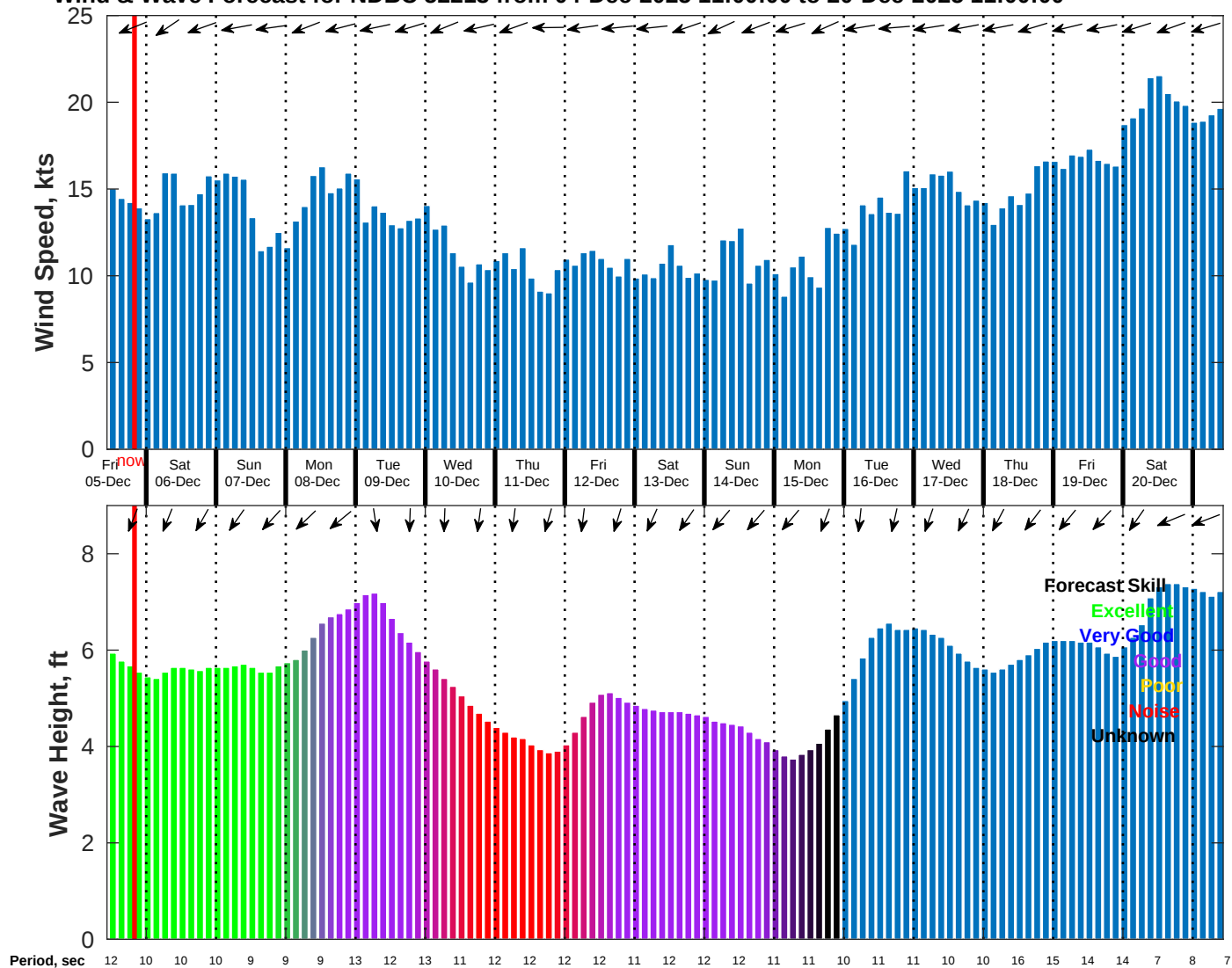
Wind & Wave Forecast for NDBC 52213 from 04-Dec-2025 11:00:00 to 20-Dec-2025 11:00:00
