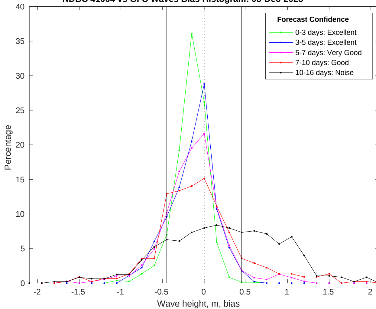
NDBC 41004 vs GFS Waves Bias Histogram: 05-Dec-2025
