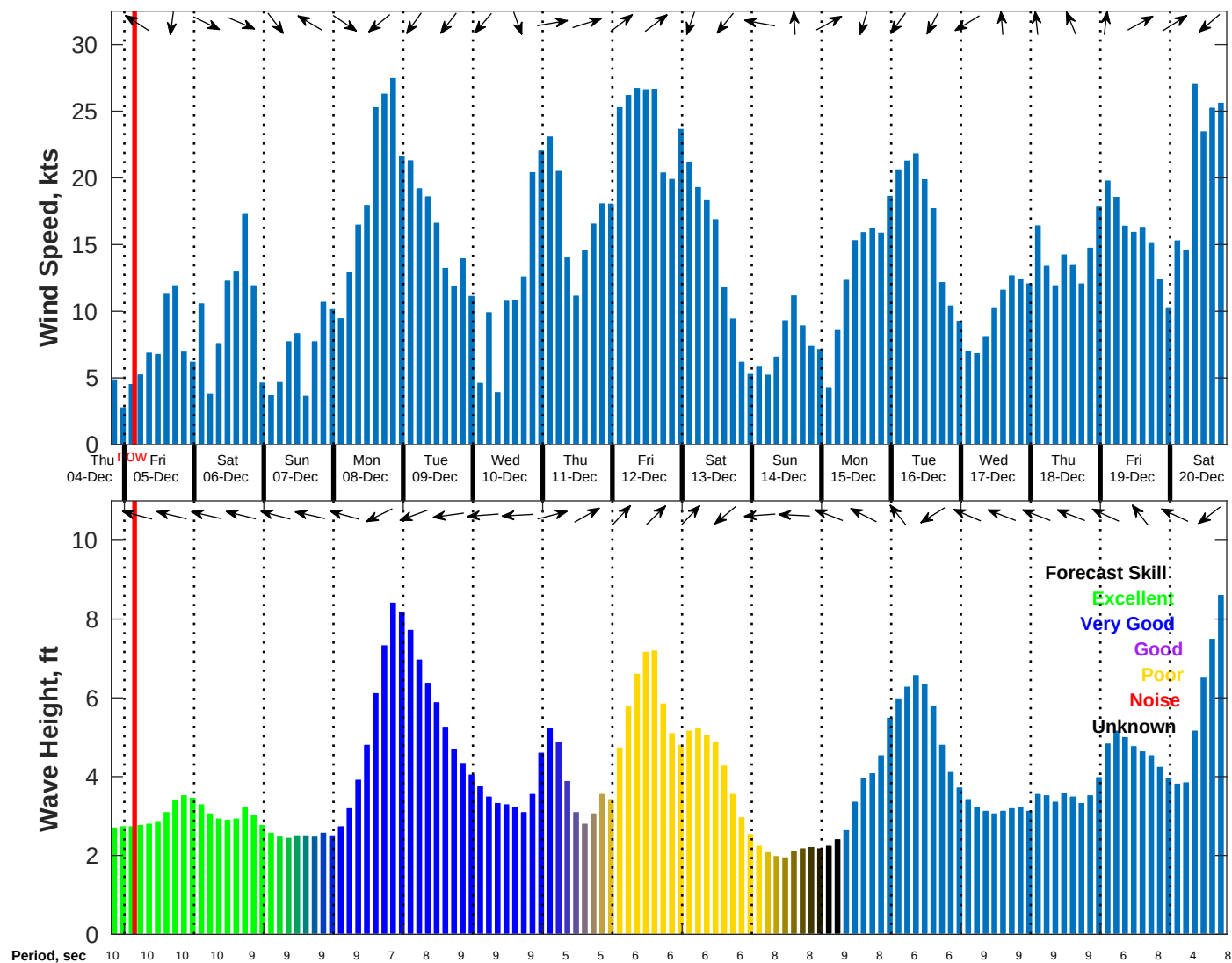
Wind & Wave Forecast for NDBC 41004 from 04-Dec-2025 19:00:00 to 20-Dec-2025 19:00:00
