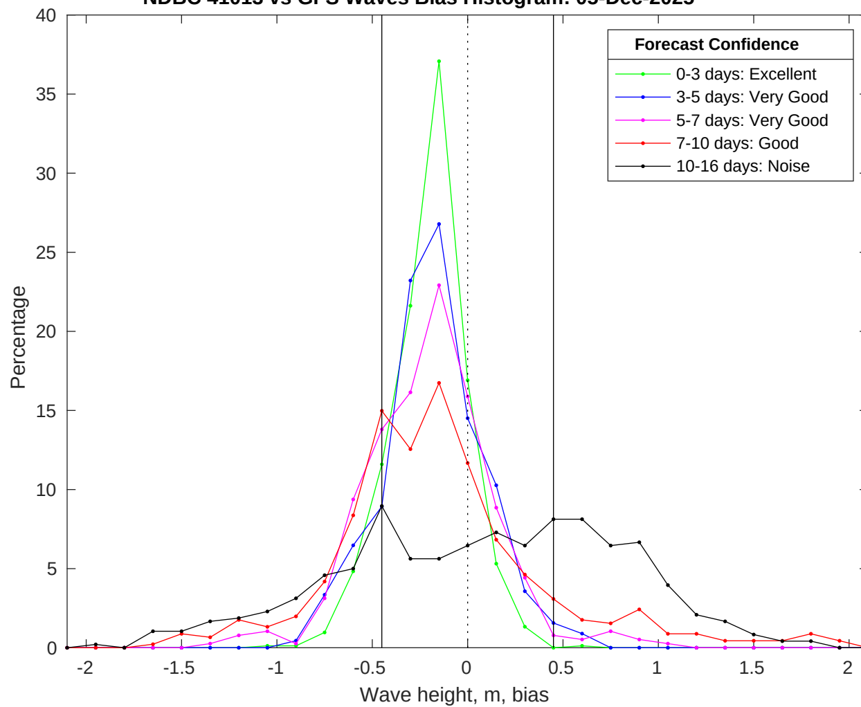
NDBC 41013 vs GFS Waves Bias Histogram: 05-Dec-2025
