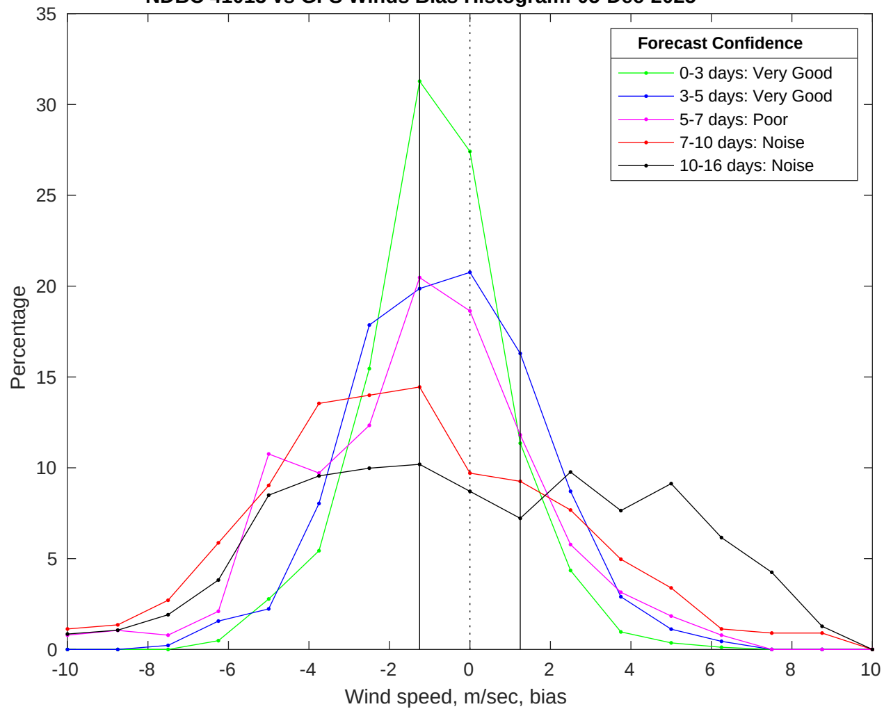
NDBC 41013 vs GFS Winds Bias Histogram: 05-Dec-2025
