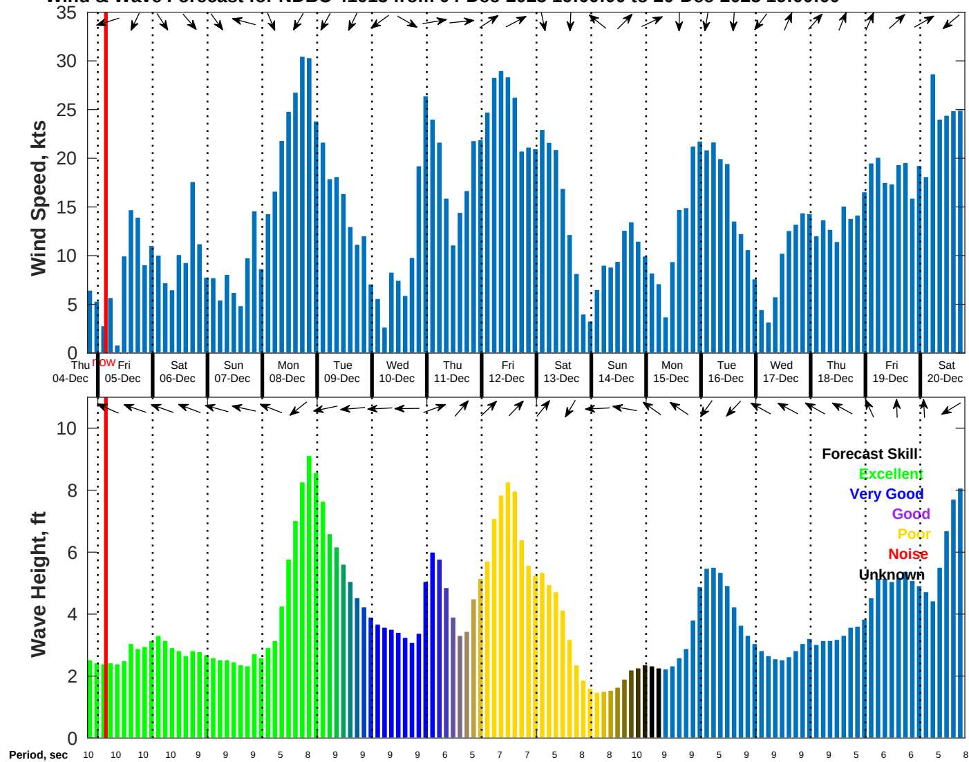
Wind & Wave Forecast for NDBC 41013 from 04-Dec-2025 19:00:00 to 20-Dec-2025 19:00:00
