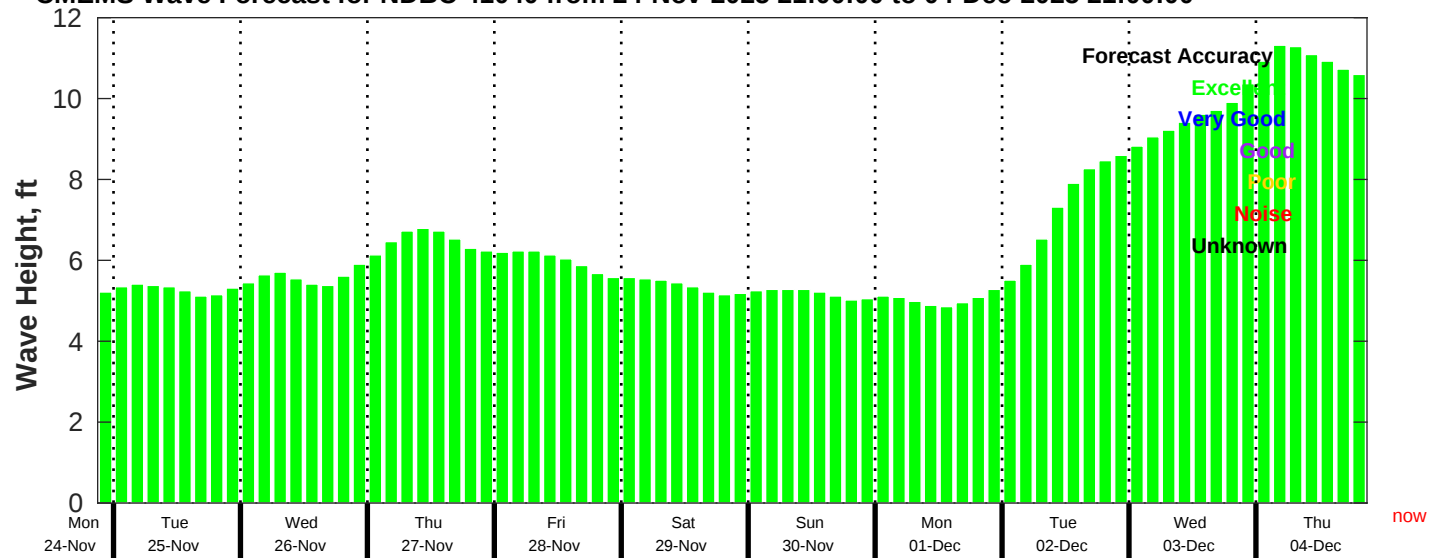
CMEMS Wave Forecast for NDBC 41040 from 24-Nov-2025 21:00:00 to 04-Dec-2025 21:00:00
