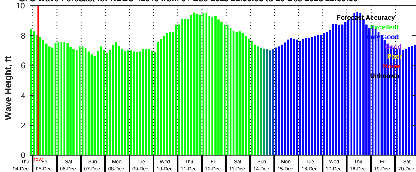
GFS Wave Forecast for NDBC 41040 from 04-Dec-2025 21:00:00 to 20-Dec-2025 21:00:00
