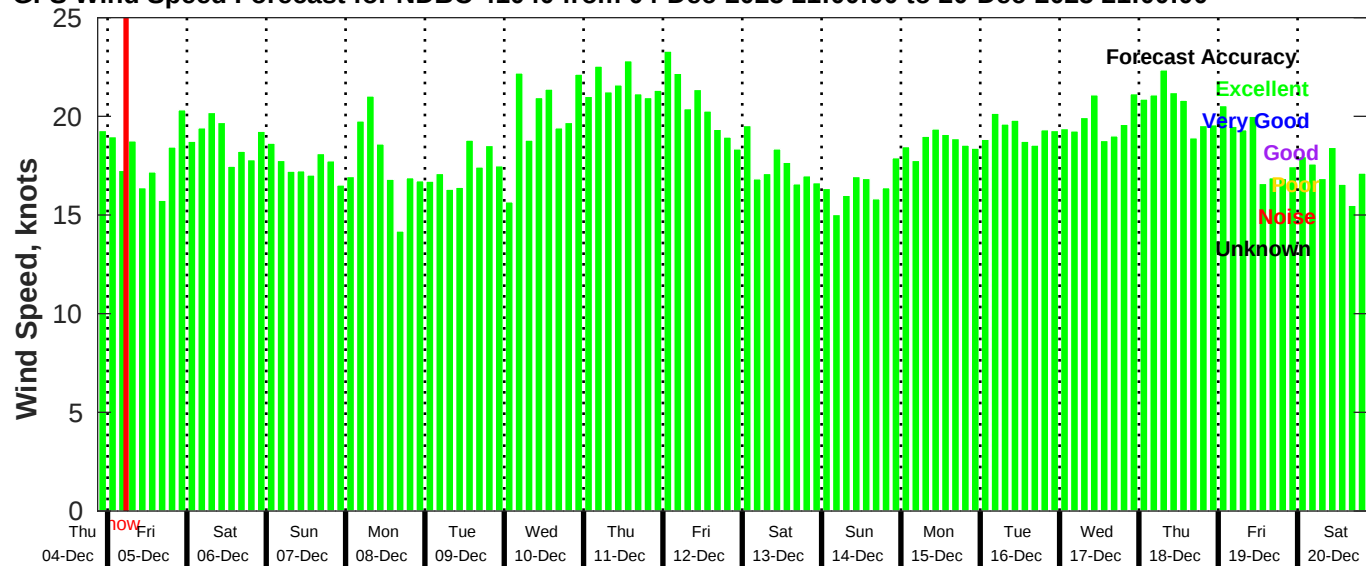
GFS Wind Speed Forecast for NDBC 41040 from 04-Dec-2025 21:00:00 to 20-Dec-2025 21:00:00
