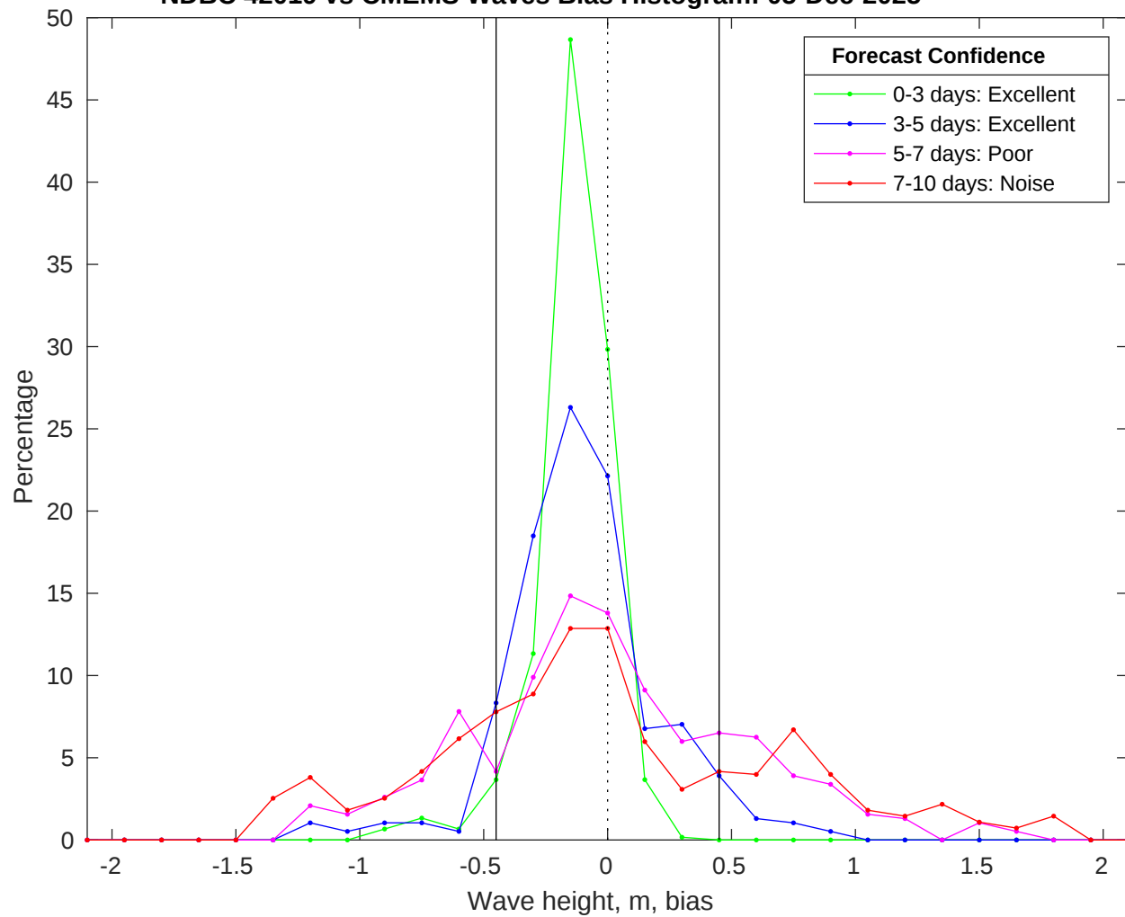
NDBC 42019 vs CMEMS Waves Bias Histogram: 05-Dec-2025
