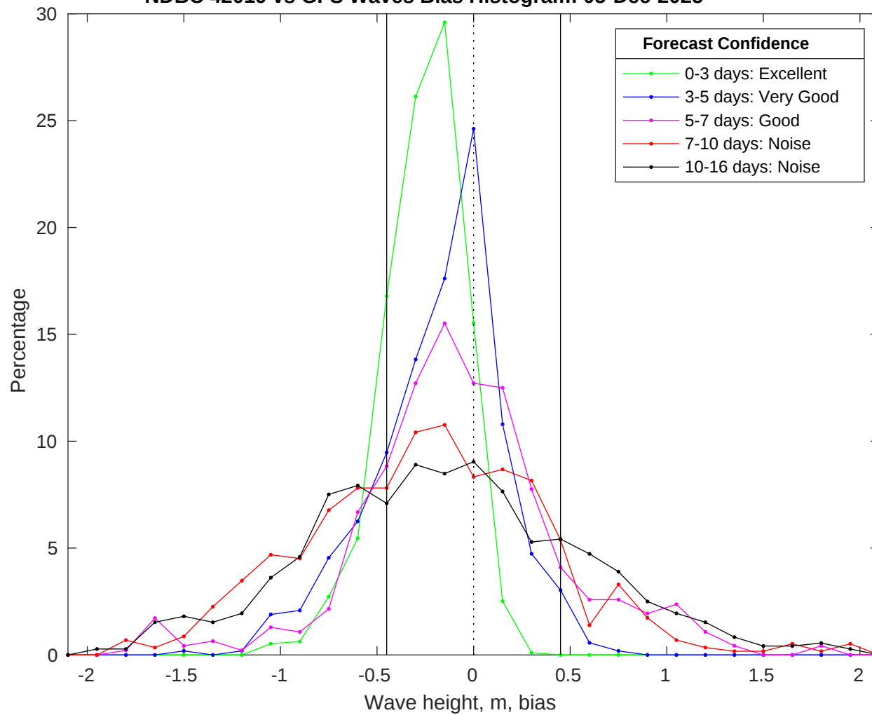
NDBC 42019 vs GFS Waves Bias Histogram: 05-Dec-2025
