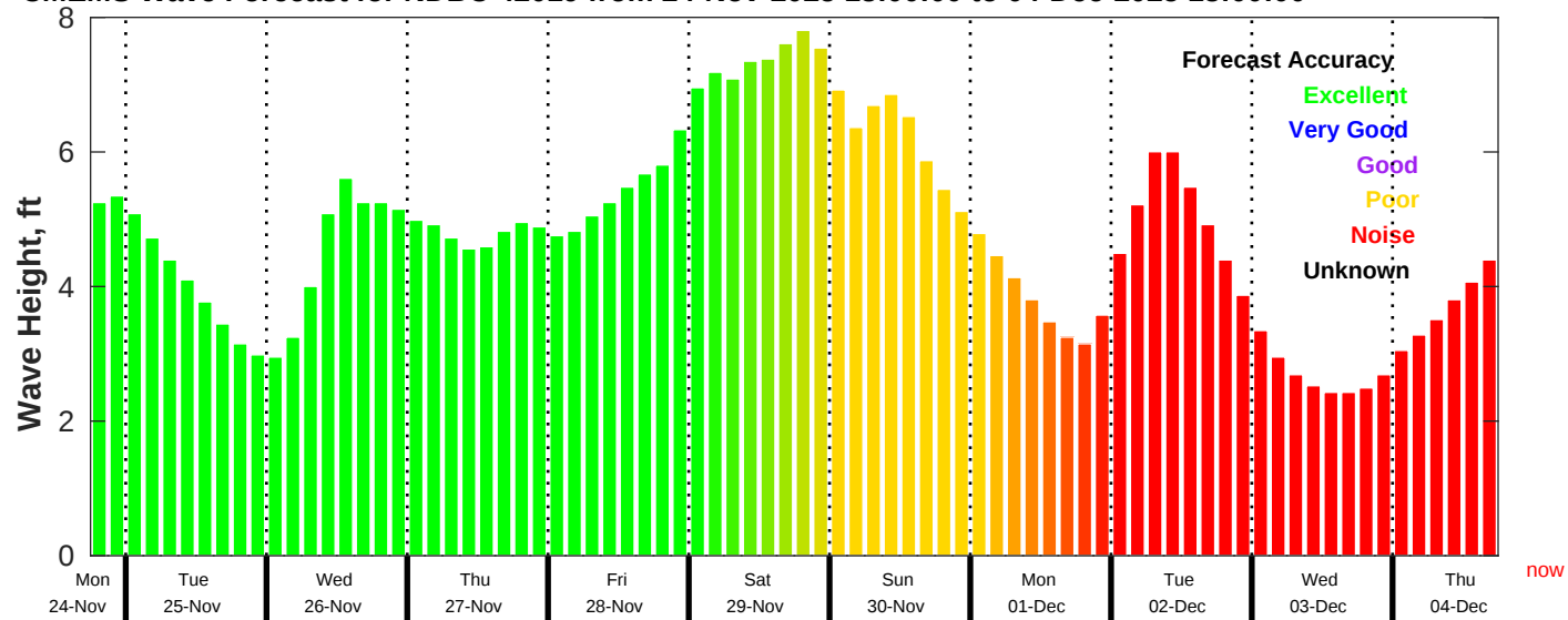
CMEMS Wave Forecast for NDBC 42019 from 24-Nov-2025 18:00:00 to 04-Dec-2025 18:00:00
