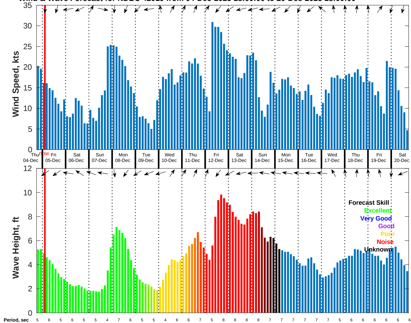
Wind & Wave Forecast for NDBC 42019 from 04-Dec-2025 18:00:00 to 20-Dec-2025 18:00:00
