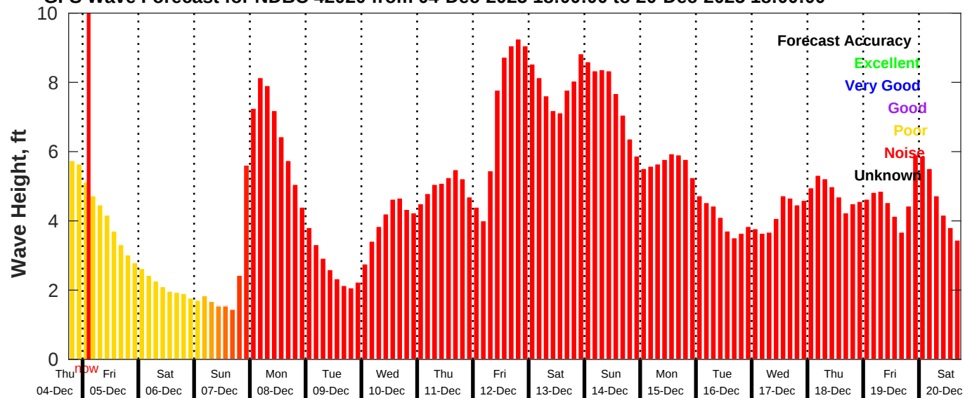
GFS Wave Forecast for NDBC 42020 from 04-Dec-2025 18:00:00 to 20-Dec-2025 18:00:00
